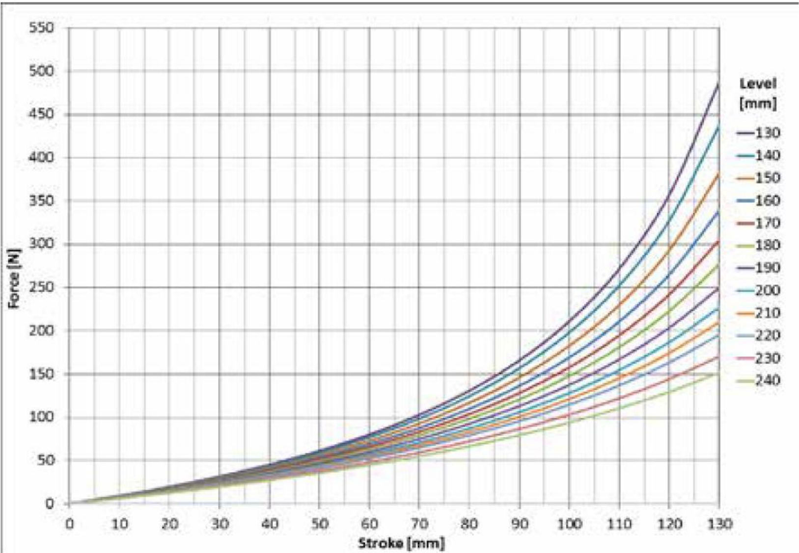
Air spring force diagram
