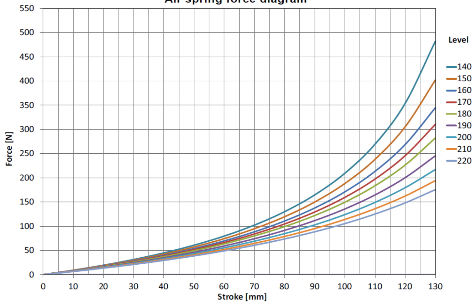
Air spring force diagram
